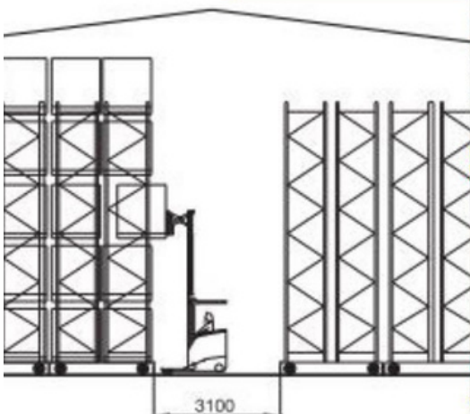
Selective Mobile Racking
